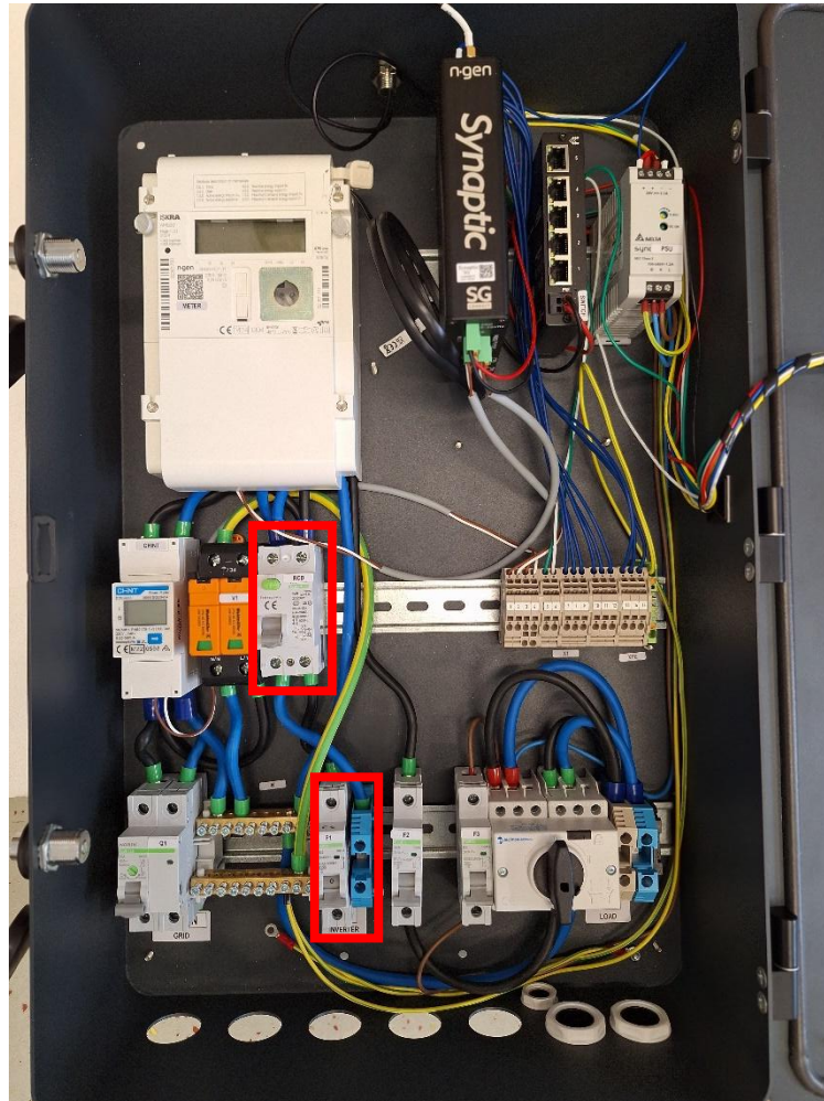
Figure 20: Switching off the Inverter fuse and RCD.
