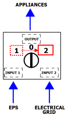
Figure 29: Changeover switch
