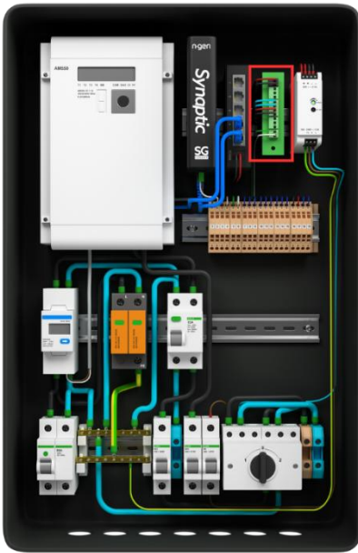
Figure 2 Smart Box A163
