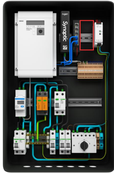
Figure 1 Smart Box B163
