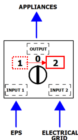
Figure 29: Changeover switch
