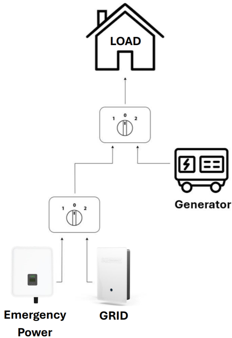
Figure 12: Connecting the generator
